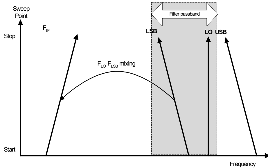
Figure 4-22 LSB Measurements
