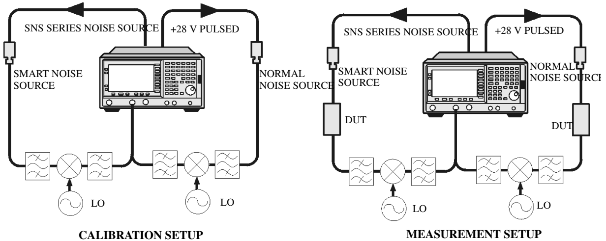
Figure 4-18 PSA System Downconverter Calibration and Measurement
