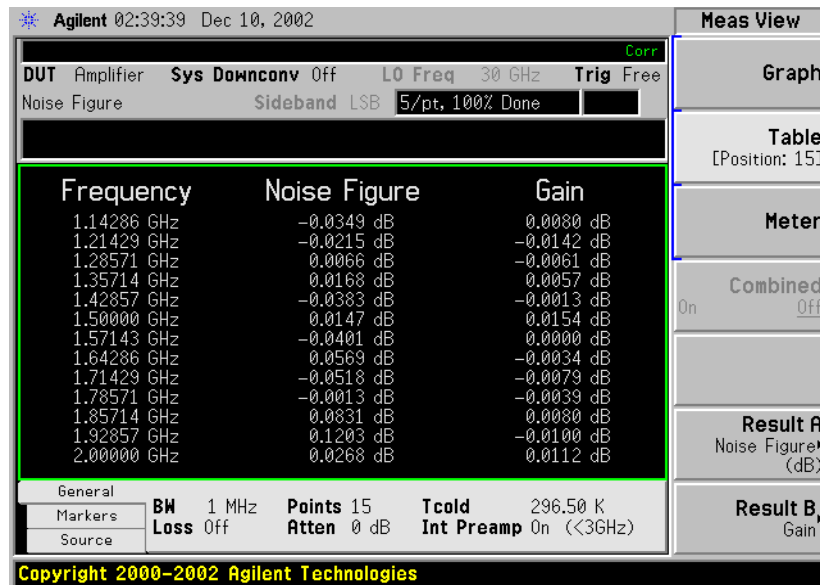
Figure 1-22 Typical Tabulated Results after Calibration
