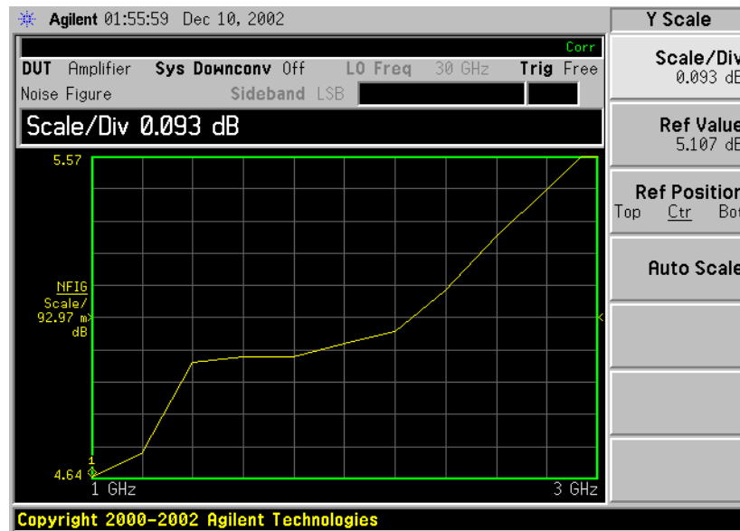
Figure 1-11 Typical Noise Figure Displayed on a Graph
