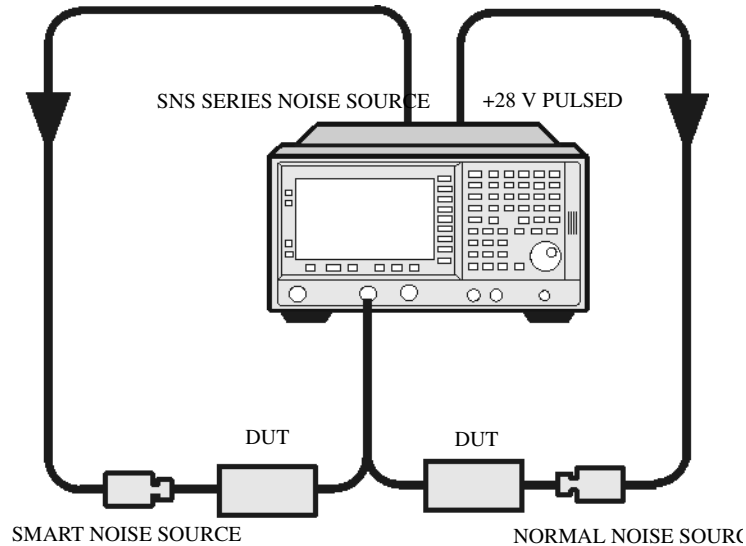
Figure 1-23 Connecting the DUT to make a measurement on an ESA
