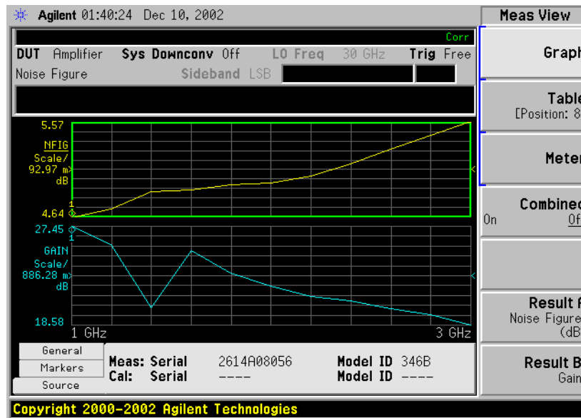
Figure 1-6 Dual-graph display
