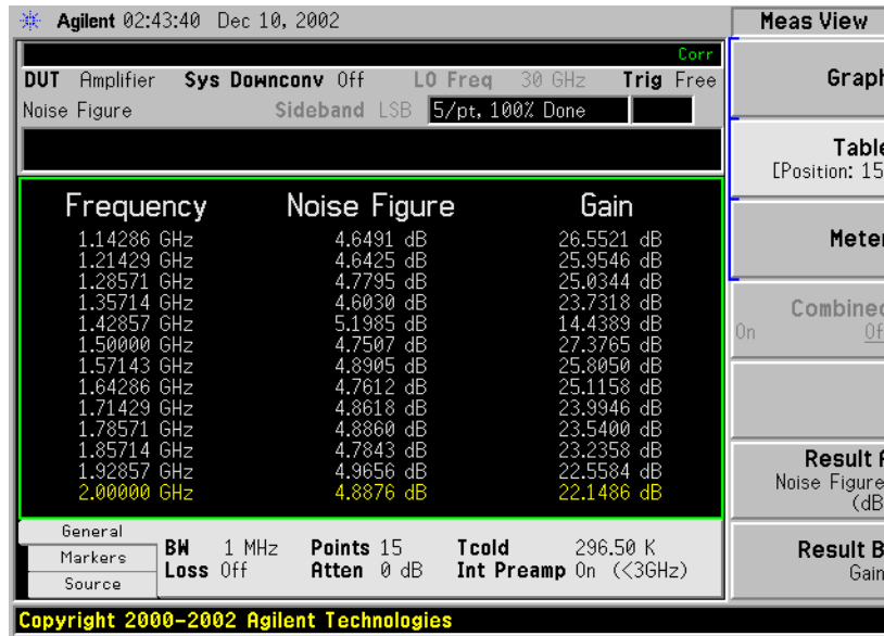
Figure 1-25 Typical Tabulated Results after Measurement
