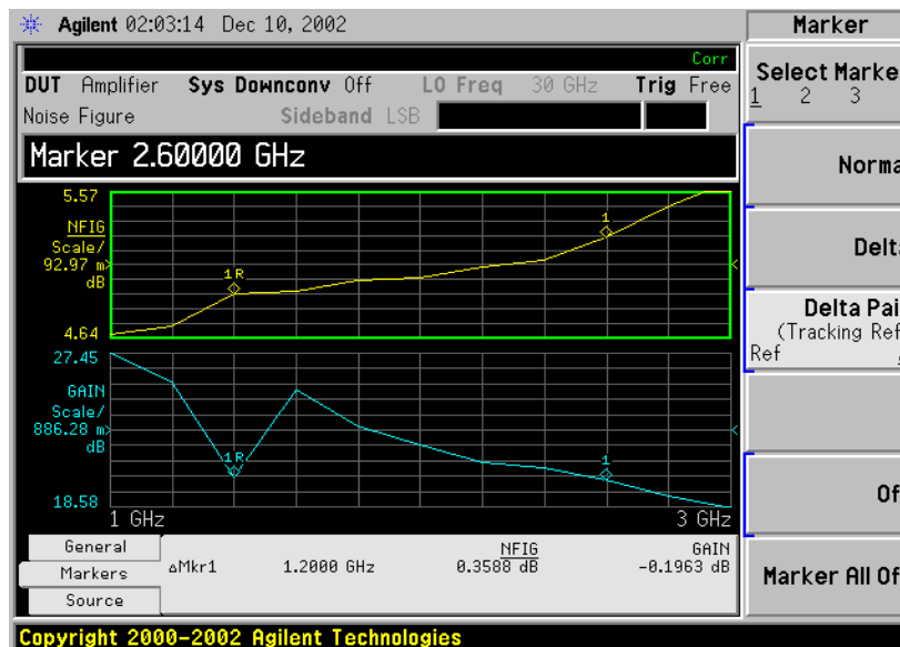
Figure 1-16 Delta Pair with Delta Marker Enabled
