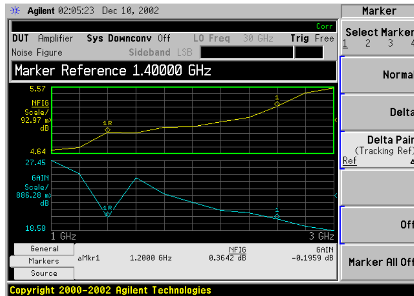
Figure 1-15 Delta Pair with Reference Marker Enabled
