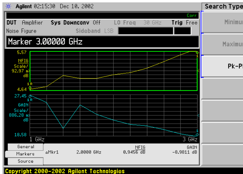
Figure 1-18 Peak to Peak Found
