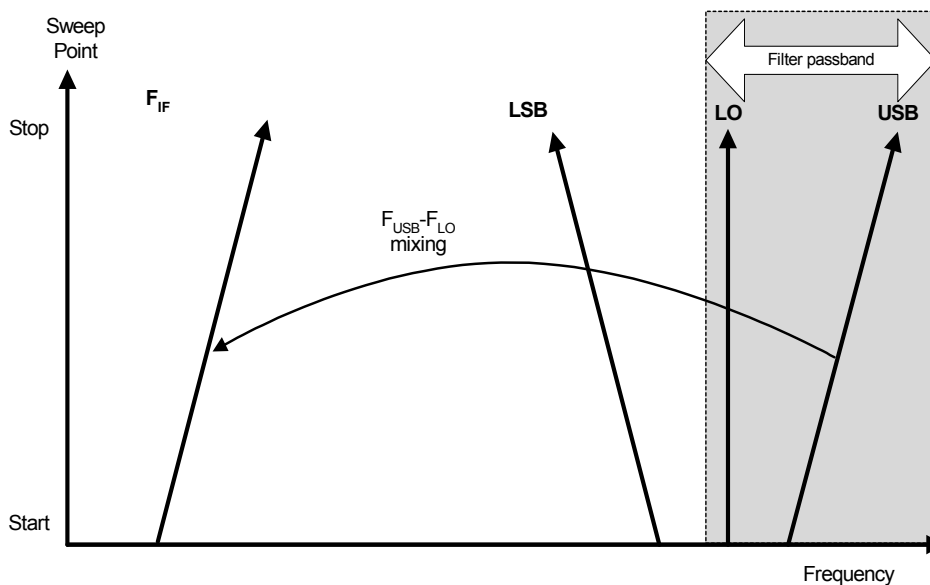
Figure 4-23 USB Measurements
