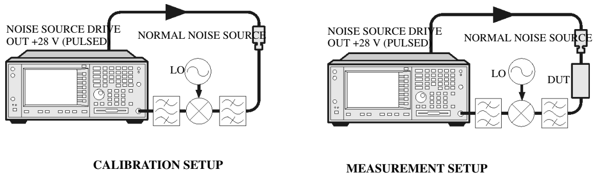
Figure 4-18 PSA System Downconverter Calibration and Measurement
