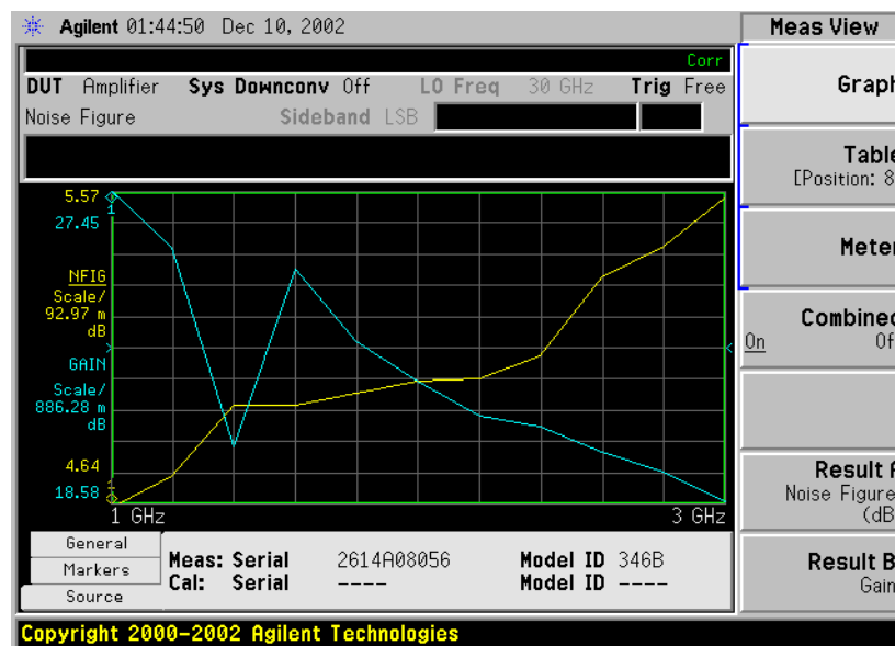
Figure 1-8 Typical display with two traces combined on the same graph
