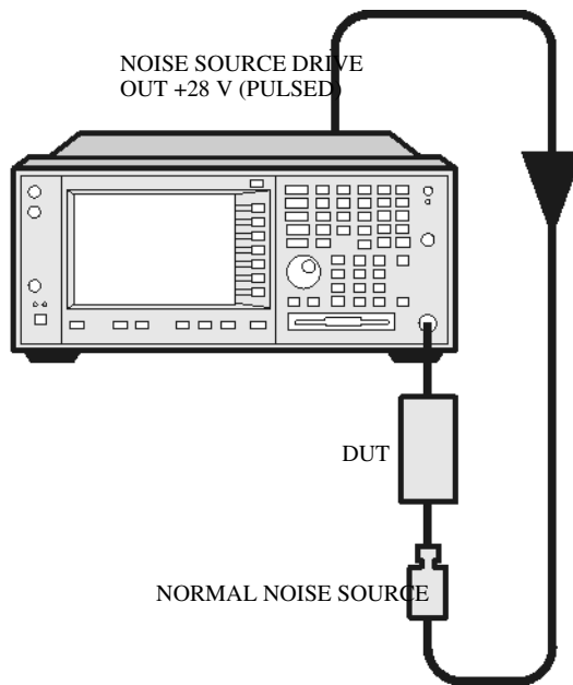
Figure 1-24 Connecting the DUT to make a measurement on a PSA
