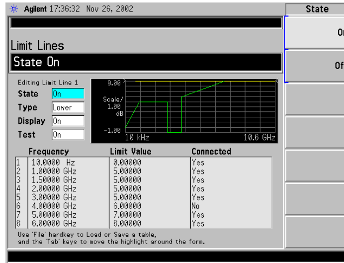
Figure 1-3 Limit Line Connections Displayed
