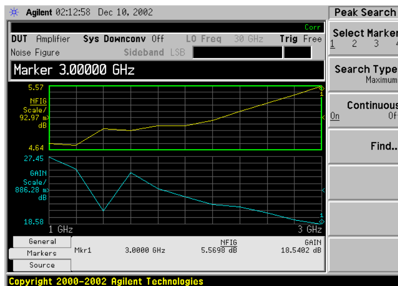
Figure 1-17 Typical Trace showing Maximum Point Found
