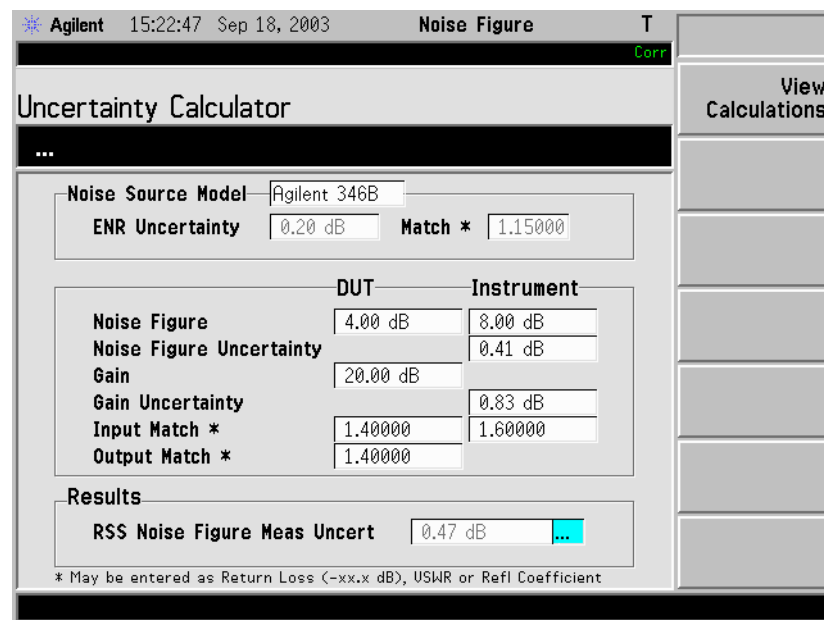
Figure 1-11 Noise Figure Uncertainty Calculator Screen
