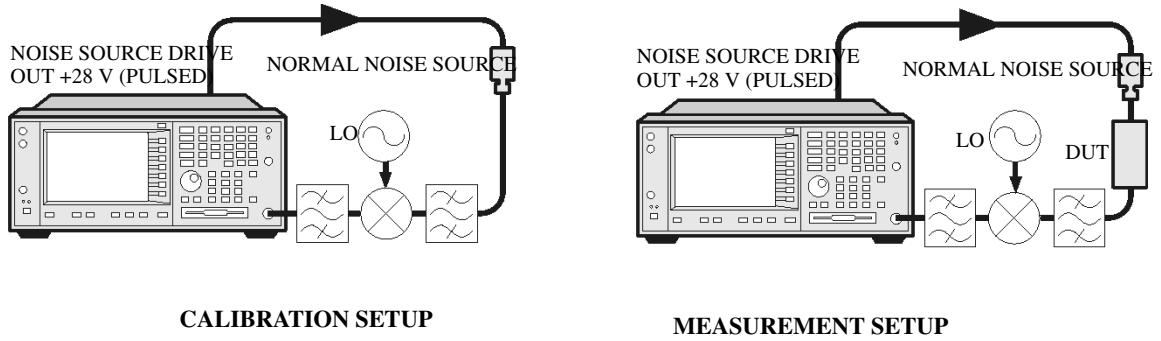
Figure 4-4 Setting Up a PSA for Frequency Converting DUT Measurement
