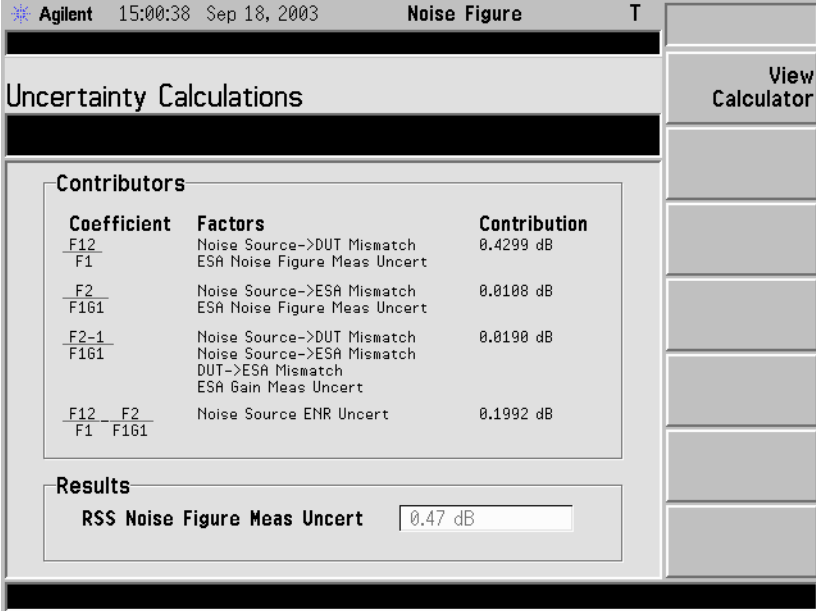
Figure 1-12 Noise Figure Uncertainty Calculations Screen
