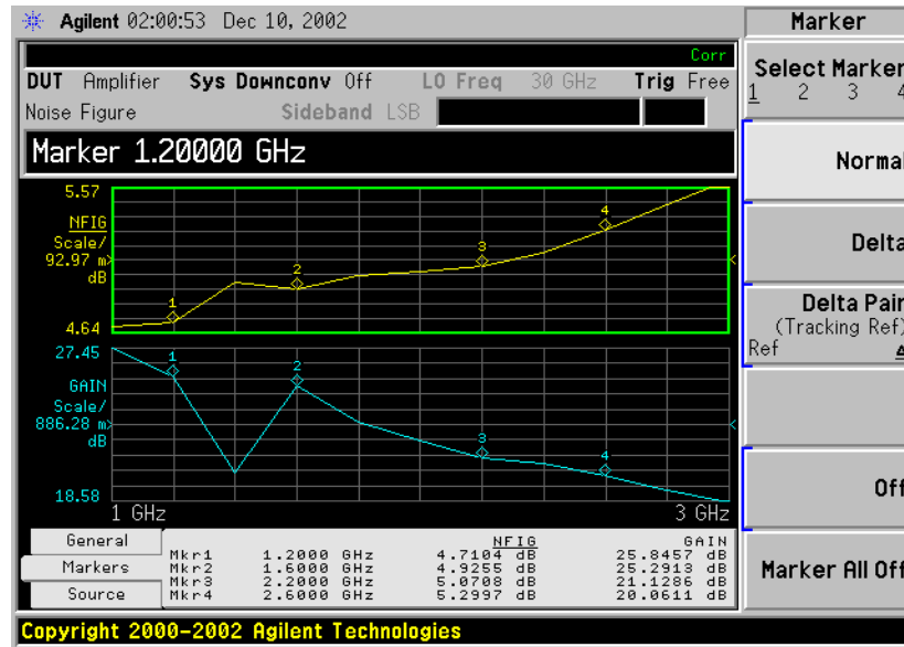
Figure 1-13 Four Normal State Markers
