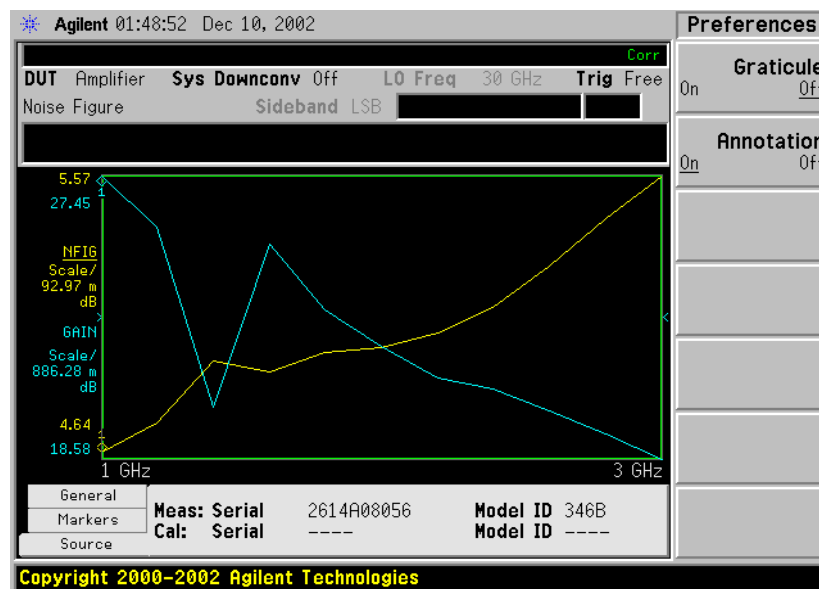
Figure 1-9 Typical Graph with Graticule Switched Off
