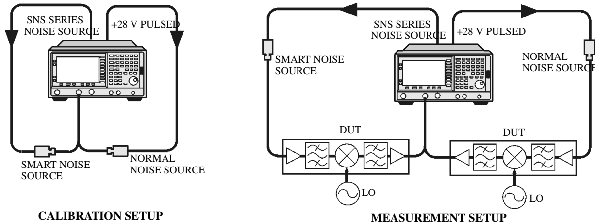
Figure 4-5 ESA Frequency Converting DUT Measurement
