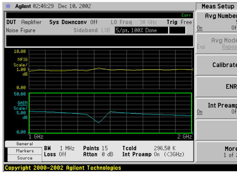
Figure 1-26 Typical Graphical Results after Measurement
