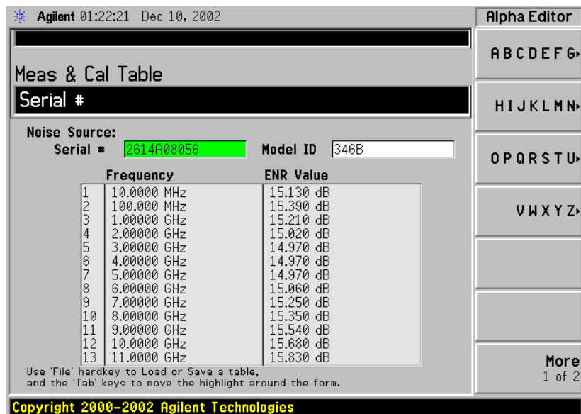
Figure 1-2 A Typical ENR Table after data entry
