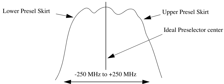
Figure 1-10 Preselector Filter Response being varied to find Optimum Frequency
