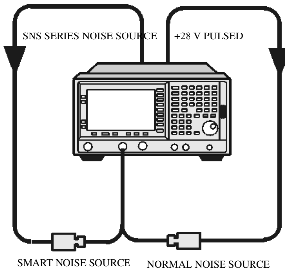
Figure 1-19 ESA Calibration Setup with Normal or Smart Noise Sources
