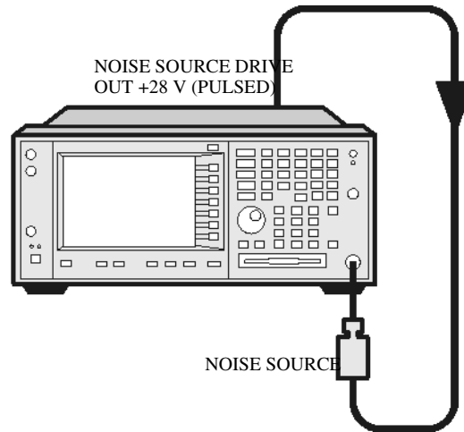
Figure 1-20 PSA Calibration Setup with Normal Noise Source
