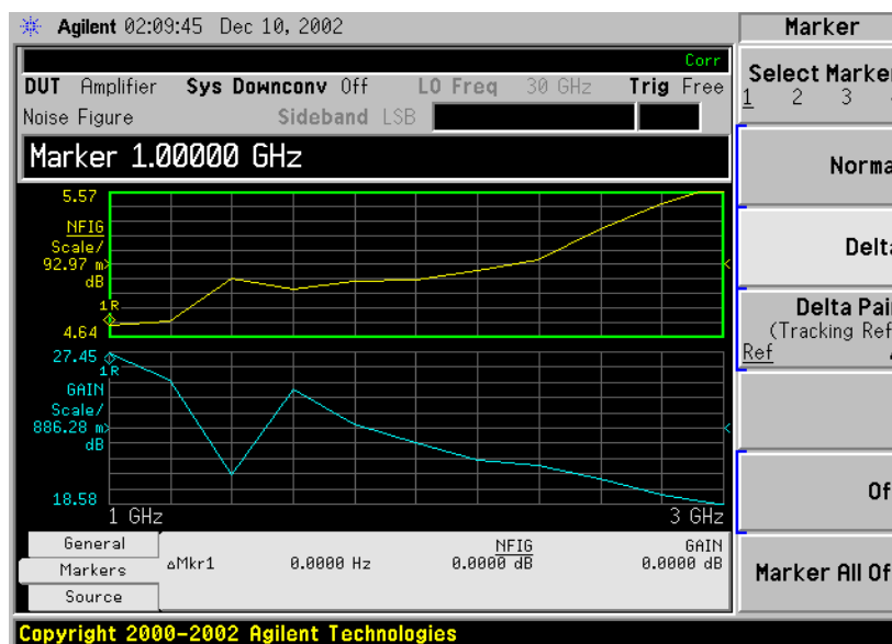
Figure 1-14 The Delta Marker State enabled
